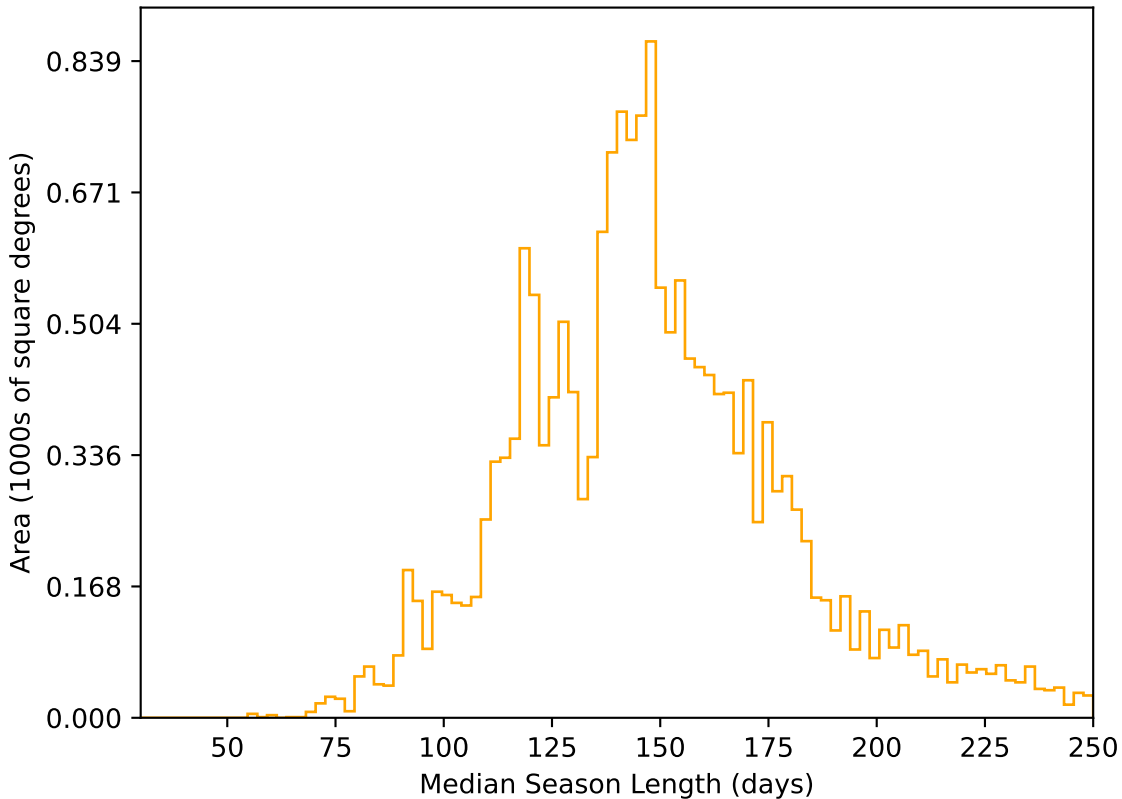
weather_cloudso20v3.4_10yrs WFD r band: Median Season Length
