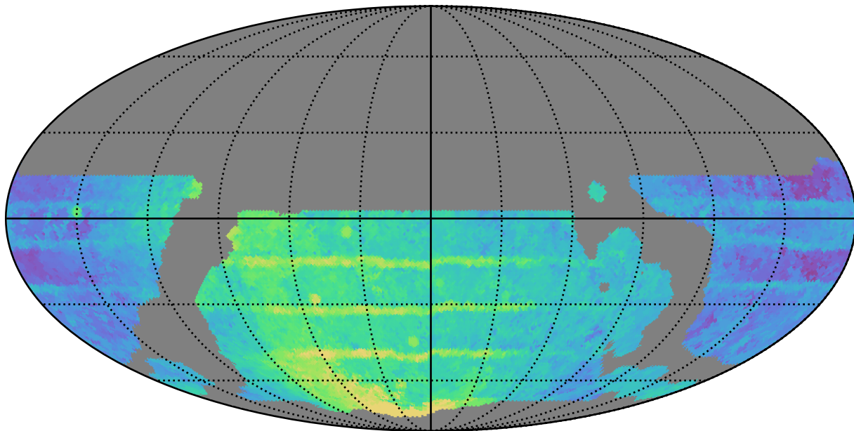
weather_cloudso20v3.4_10yrs WFD i band: Median Season Length
