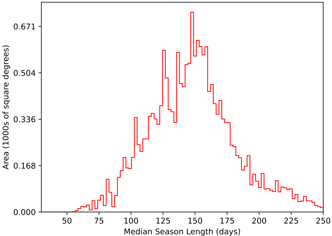
weather_cloudso20v3.4_10yrs WFD i band: Median Season Length
