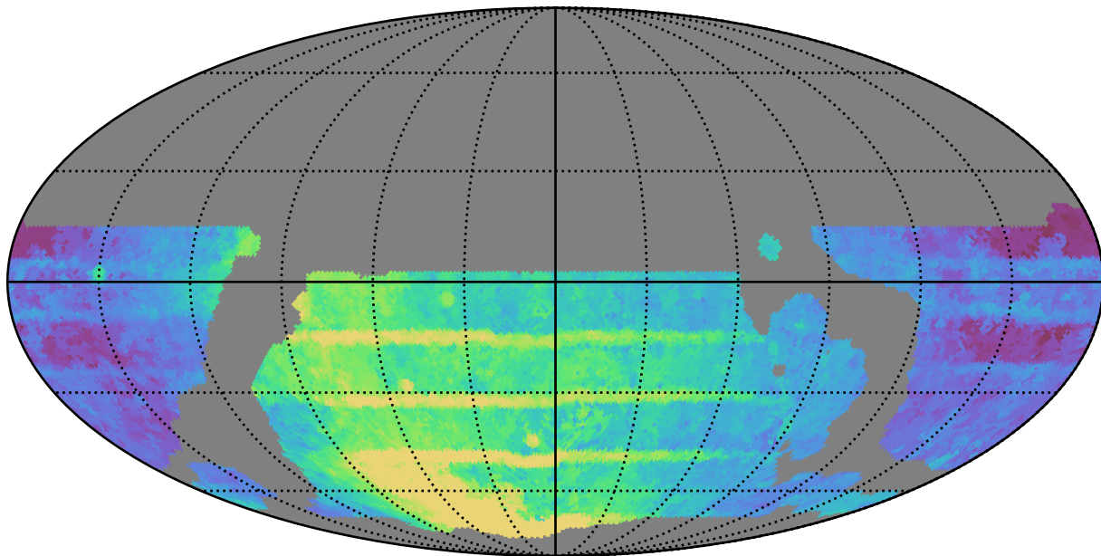
weather_cloudso20v3.4_10yrs WFD all bands: Median Season Length
