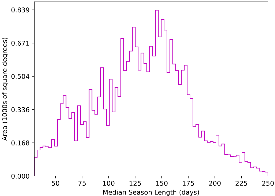
weather_cloudso20v3.4_10yrs All sky z band: Median Season Length
