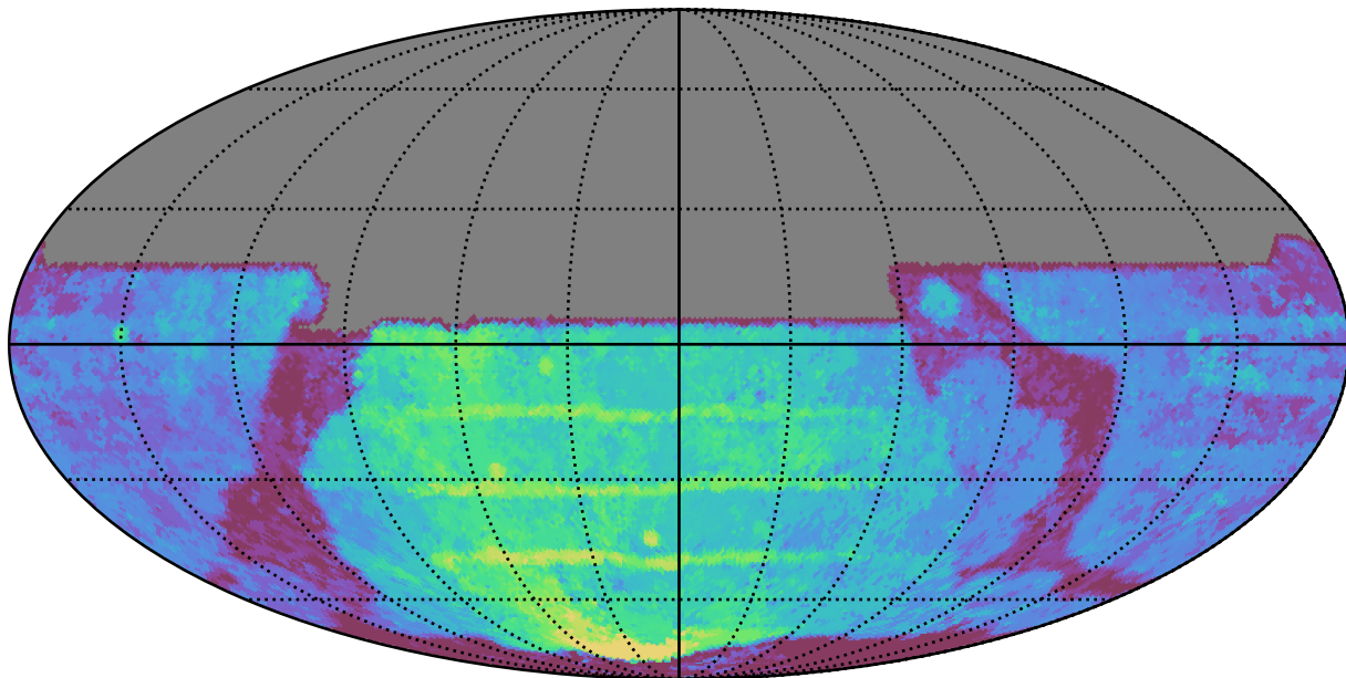
weather_cloudso20v3.4_10yrs All sky y band: Median Season Length
