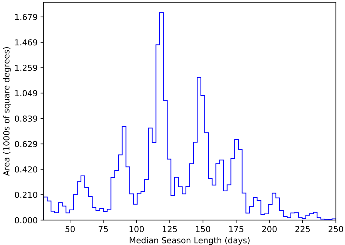
weather_cloudso20v3.4_10yrs All sky y band: Median Season Length
