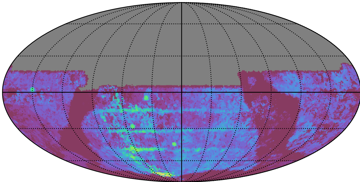
weather_cloudso20v3.4_10yrs All sky u band: Median Season Length
