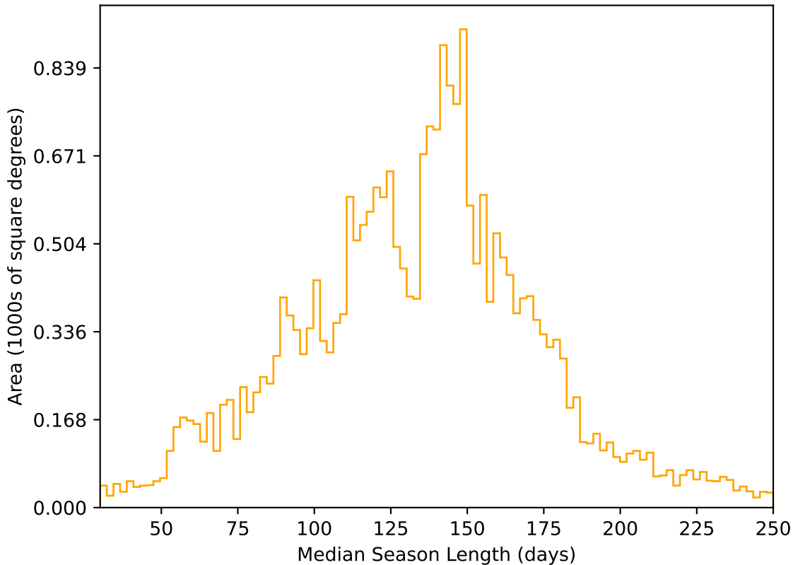
weather_cloudso20v3.4_10yrs All sky r band: Median Season Length
