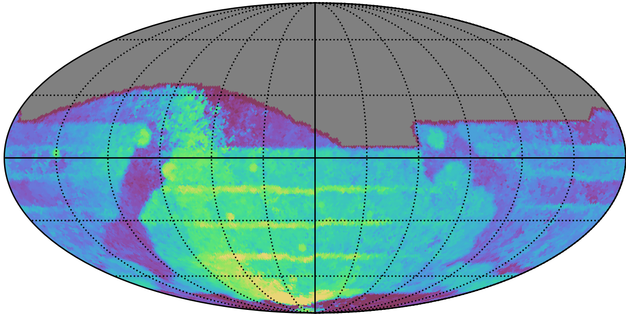
weather_cloudso20v3.4_10yrs All sky i band: Median Season Length
