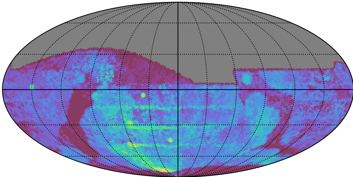
weather_cloudso20v3.4_10yrs All sky g band: Median Season Length
