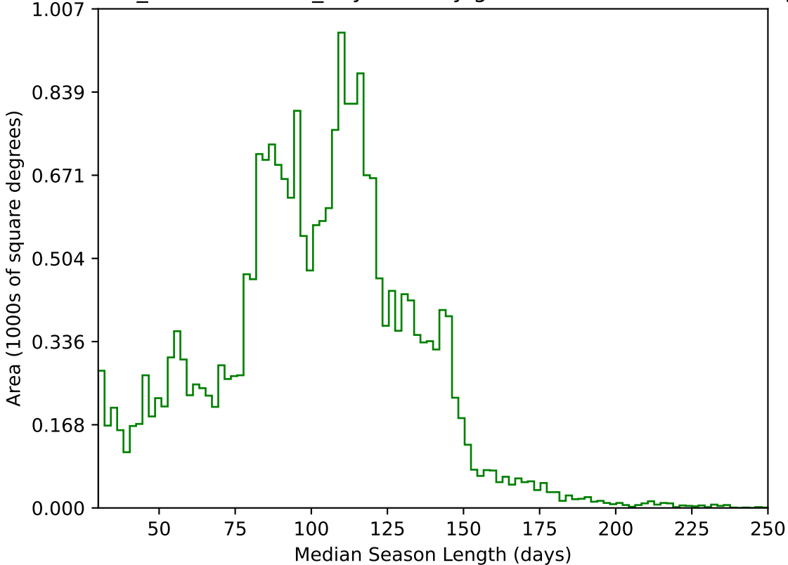
weather_cloudso20v3.4_10yrs All sky g band: Median Season Length
