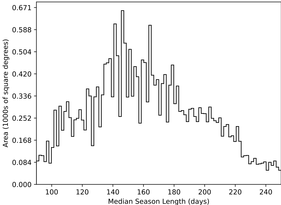
weather_cloudso20v3.4_10yrs All sky all bands: Median Season Length
