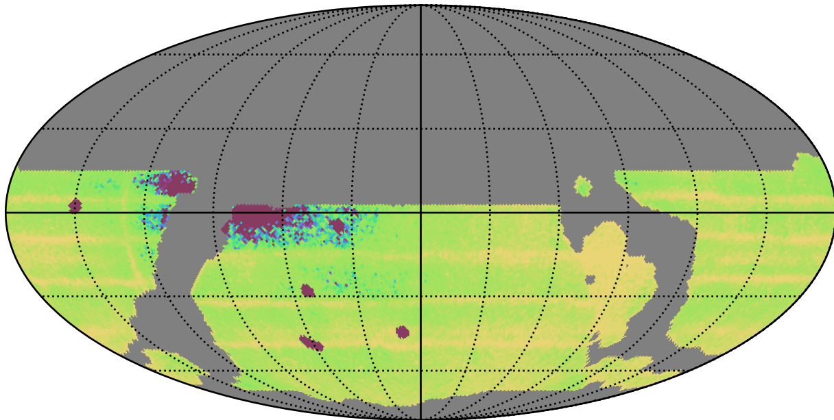
weather_cloudso20v3.4_10yrs WFD: Median Intra-Night Gap
