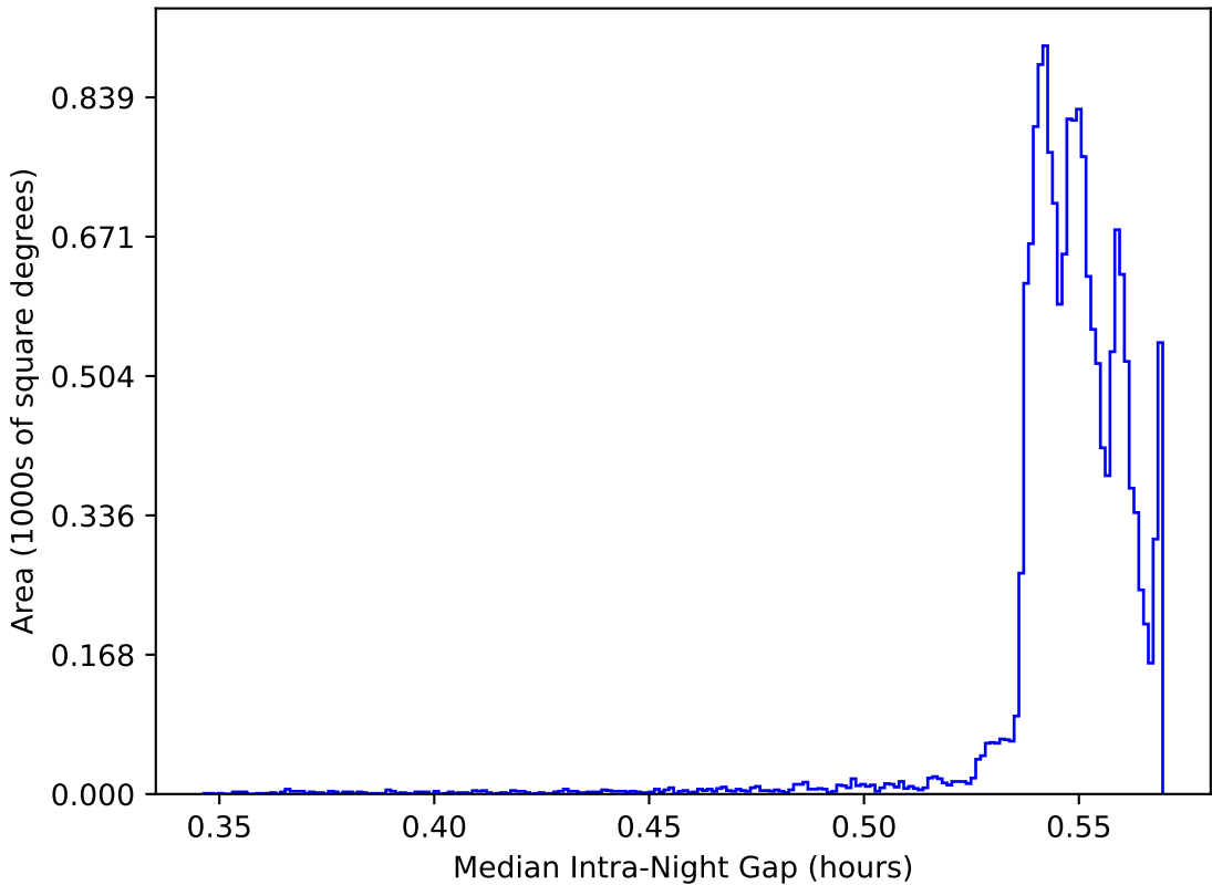
weather_cloudso20v3.4_10yrs WFD: Median Intra-Night Gap
