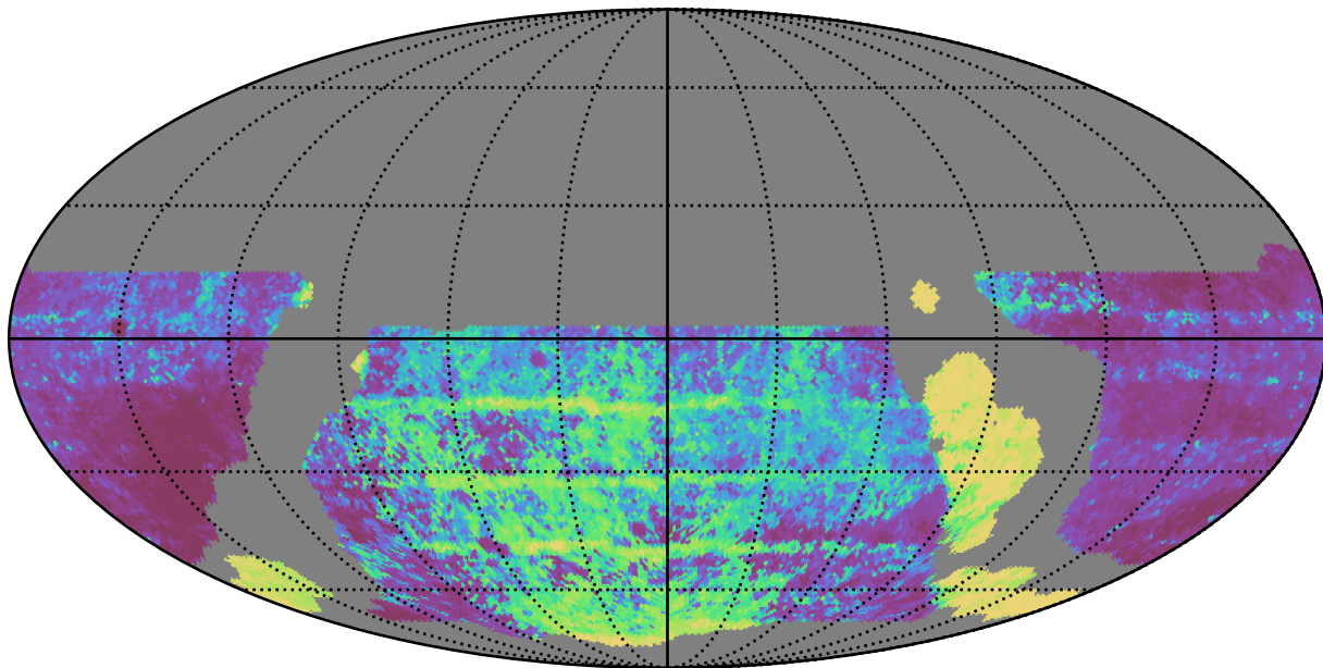
weather_cloudso20v3.4_10yrs WFD y band: Median Inter-Night Gap
