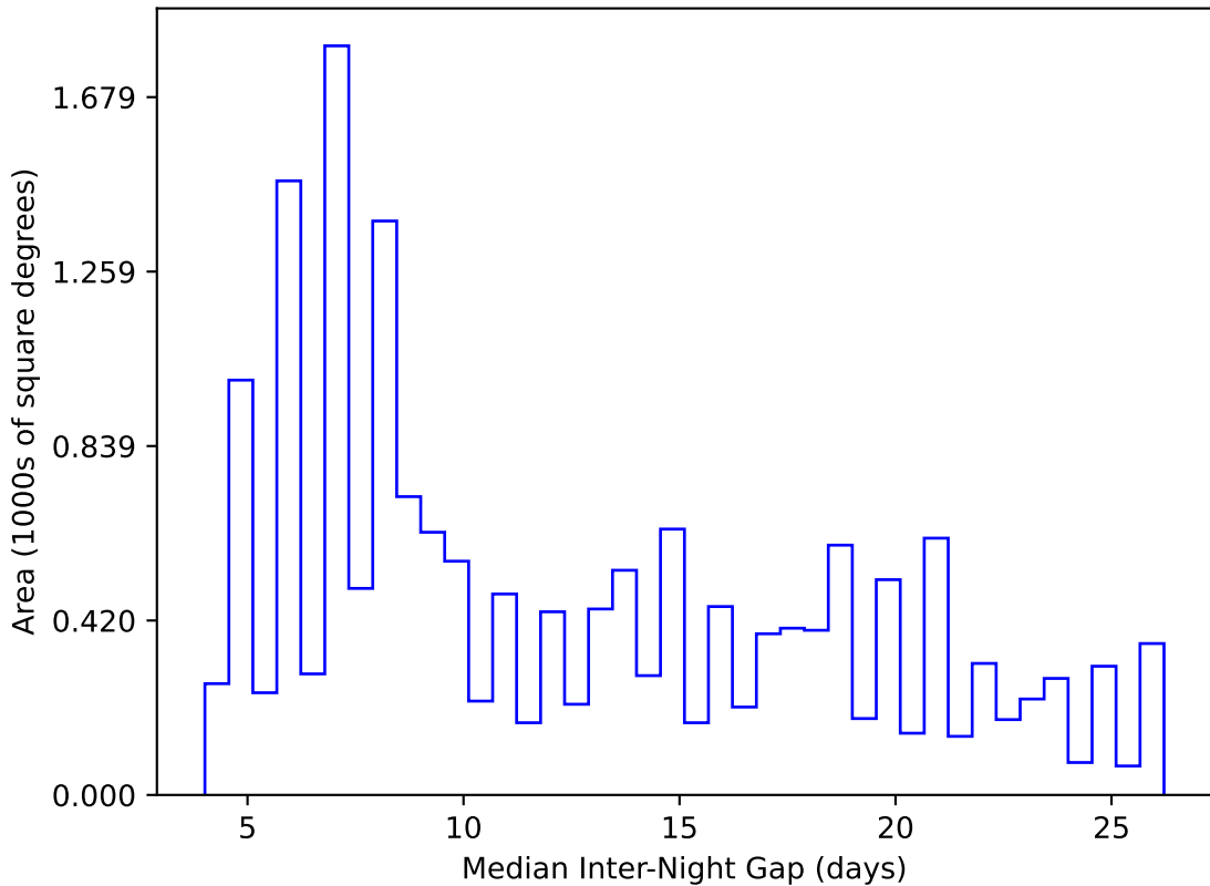
weather_cloudso20v3.4_10yrs WFD y band: Median Inter-Night Gap
