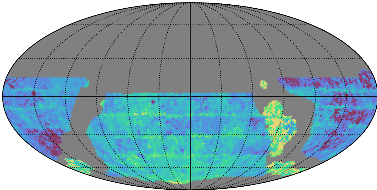
weather_cloudso20v3.4_10yrs WFD u band: Median Inter-Night Gap
