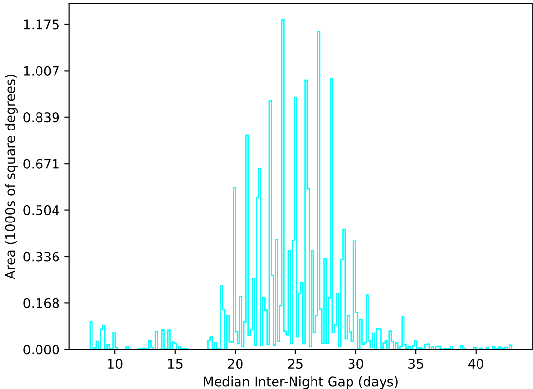
weather_cloudso20v3.4_10yrs WFD u band: Median Inter-Night Gap
