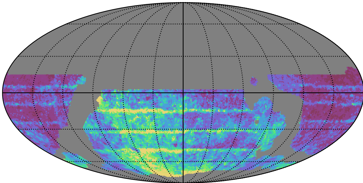
weather_cloudso20v3.4_10yrs WFD r band: Median Inter-Night Gap
