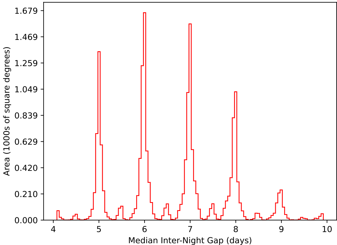
weather_cloudso20v3.4_10yrs WFD i band: Median Inter-Night Gap
