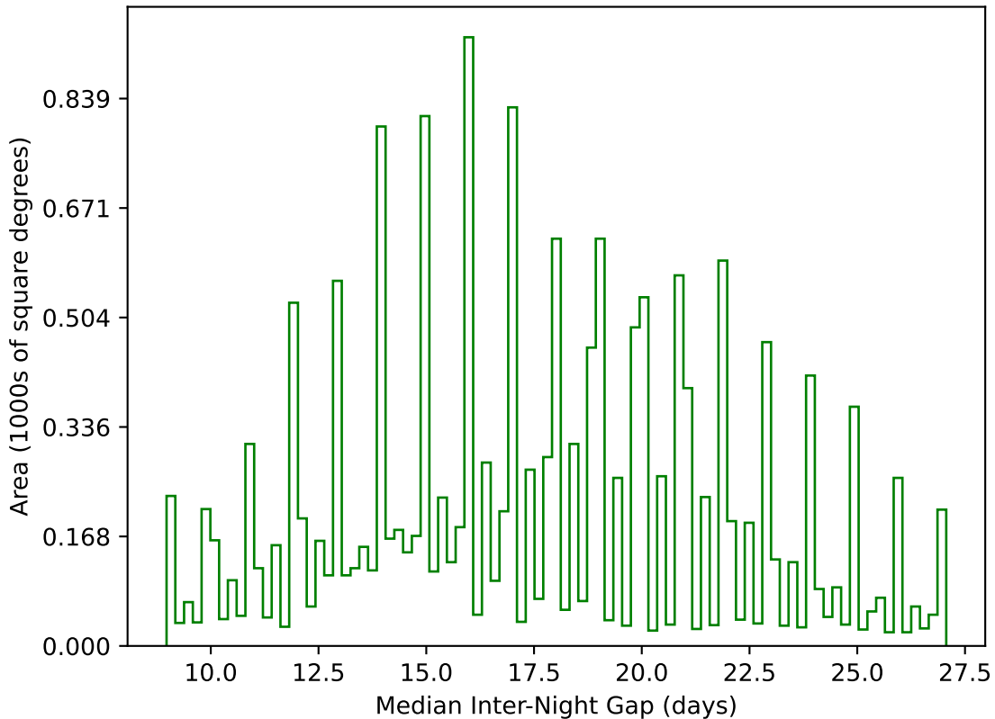
weather_cloudso20v3.4_10yrs WFD g band: Median Inter-Night Gap
