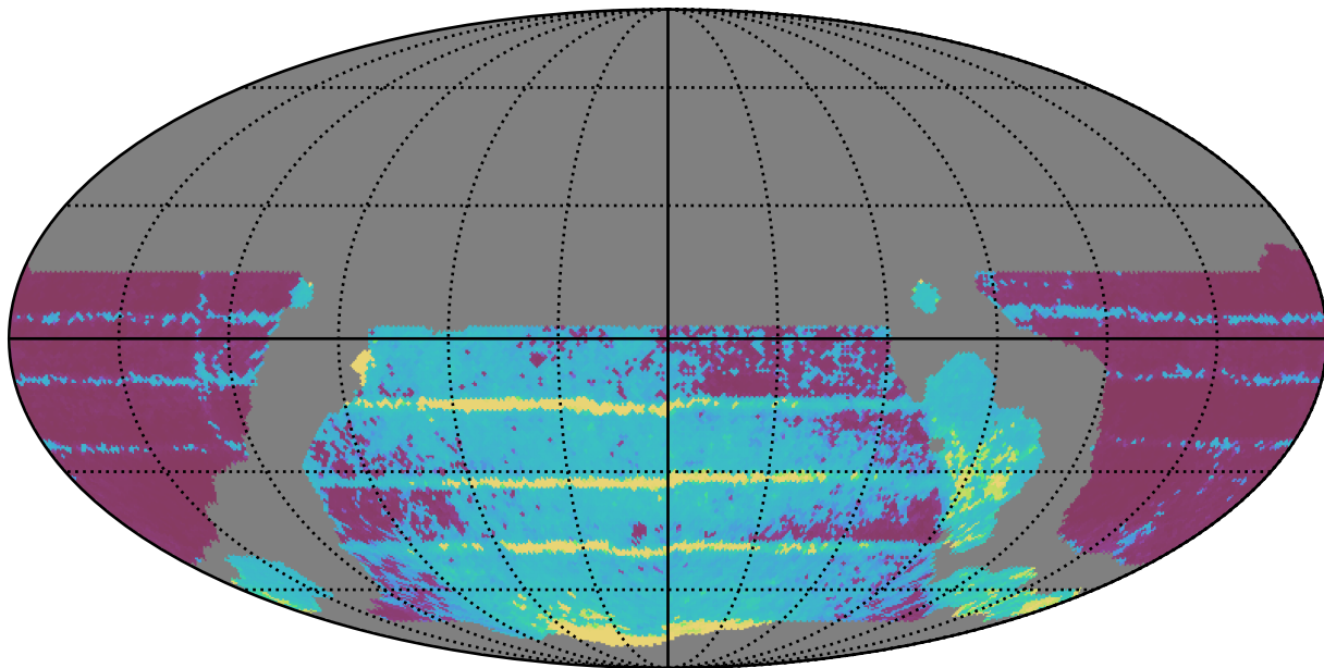
weather_cloudso20v3.4_10yrs WFD all bands: Median Inter-Night Gap
