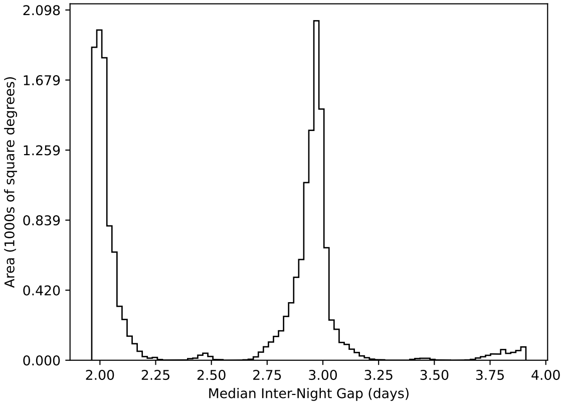
weather_cloudso20v3.4_10yrs WFD all bands: Median Inter-Night Gap
