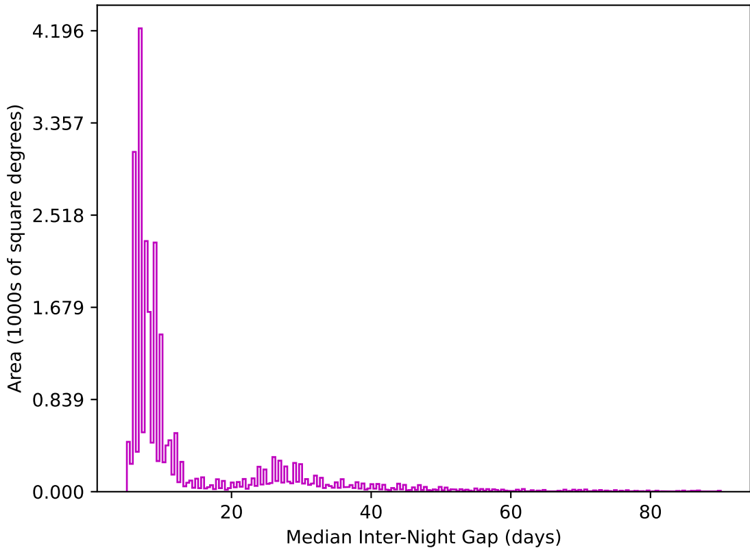
weather_cloudso20v3.4_10yrs All sky z band: Median Inter-Night Gap
