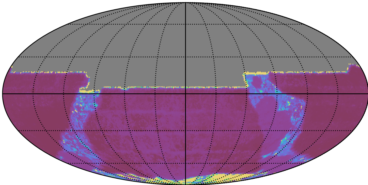
weather_cloudso20v3.4_10yrs All sky y band: Median Inter-Night Gap
