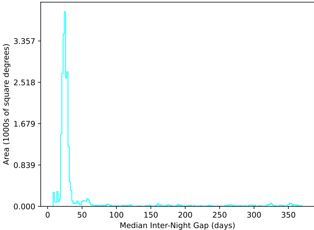
weather_cloudso20v3.4_10yrs All sky u band: Median Inter-Night Gap
