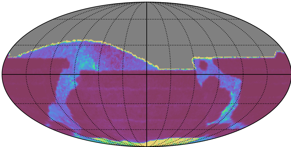
weather_cloudso20v3.4_10yrs All sky r band: Median Inter-Night Gap
