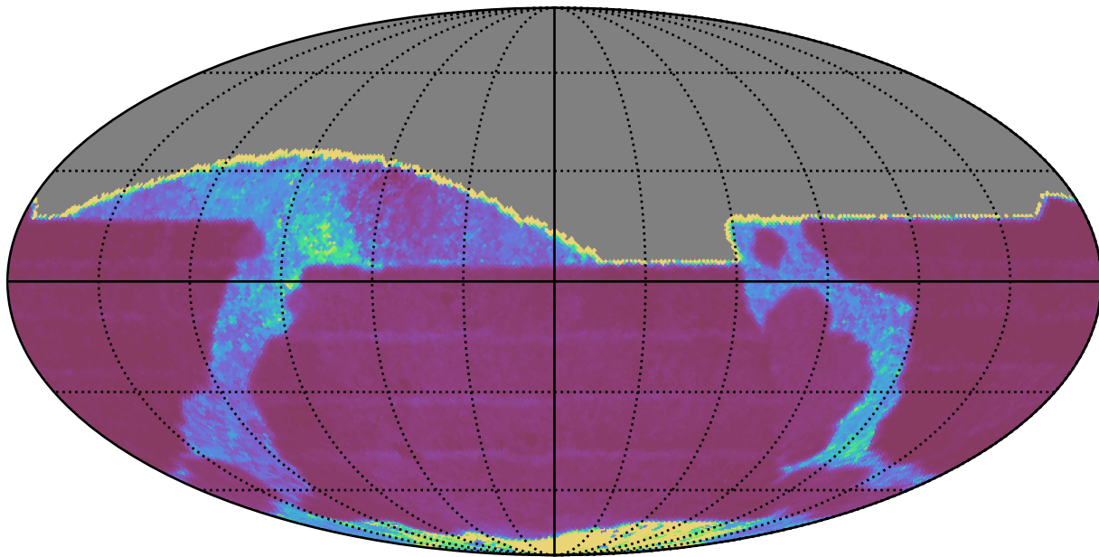
weather_cloudso20v3.4_10yrs All sky i band: Median Inter-Night Gap
