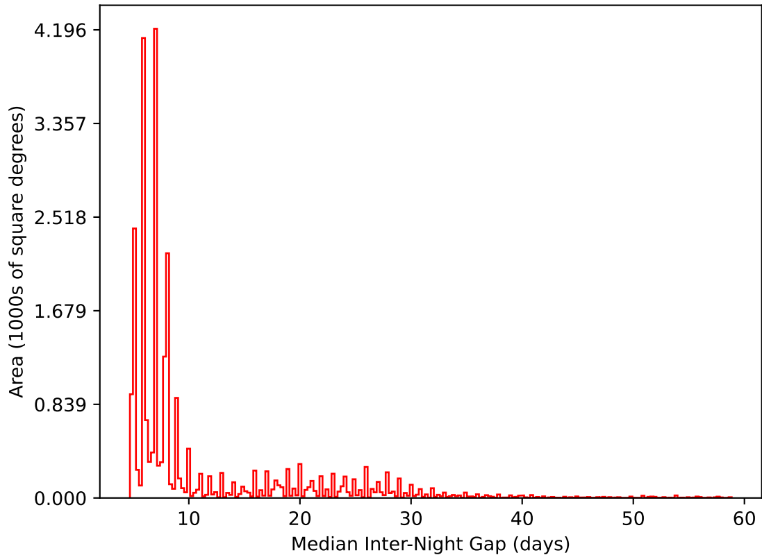
weather_cloudso20v3.4_10yrs All sky i band: Median Inter-Night Gap
