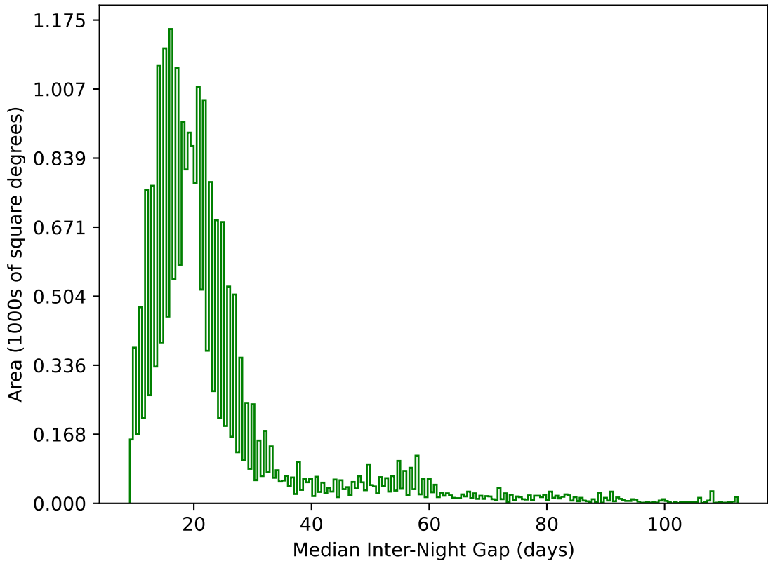
weather_cloudso20v3.4_10yrs All sky g band: Median Inter-Night Gap
