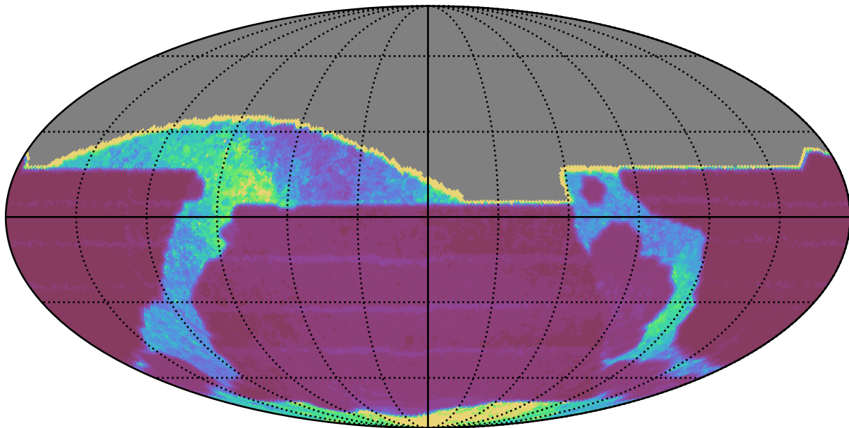
weather_cloudso20v3.4_10yrs All sky all bands: Median Inter-Night Gap
