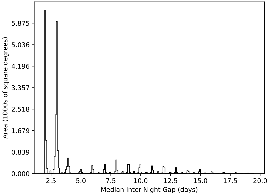
weather_cloudso20v3.4_10yrs All sky all bands: Median Inter-Night Gap
