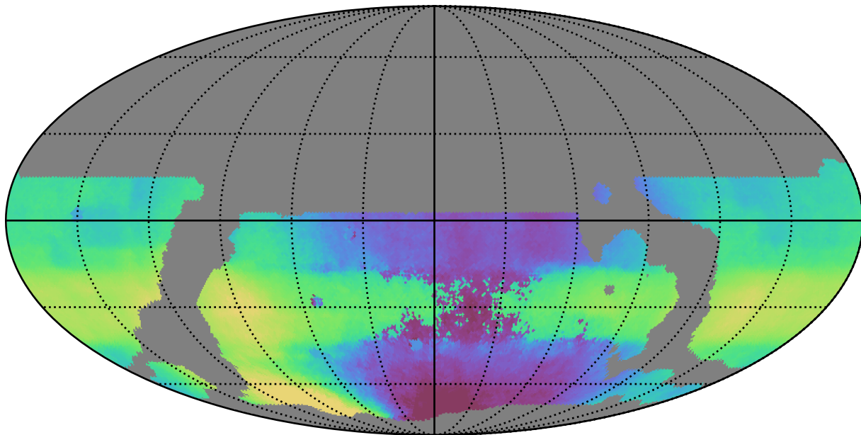
weather_cloudso20v3.4_10yrs WFD all bands: Median HA
