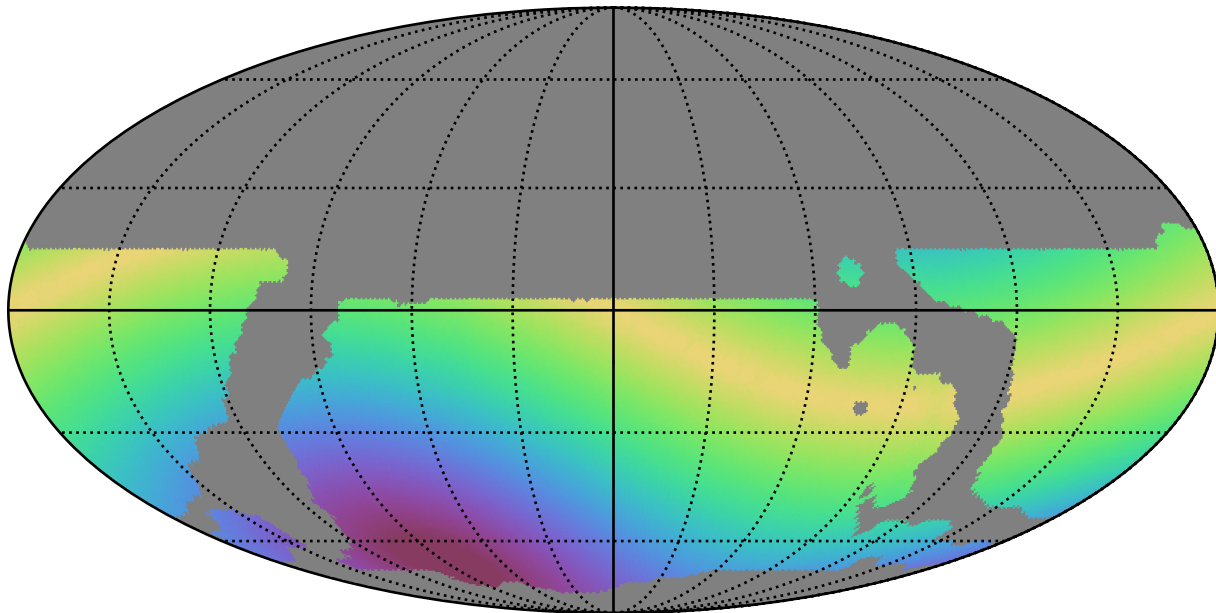
weather_cloudso20v3.4_10yrs WFD all bands: Max solarElong
