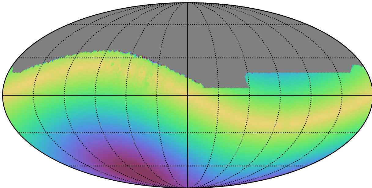
weather_cloudso20v3.4_10yrs All sky all bands: Max solarElong
