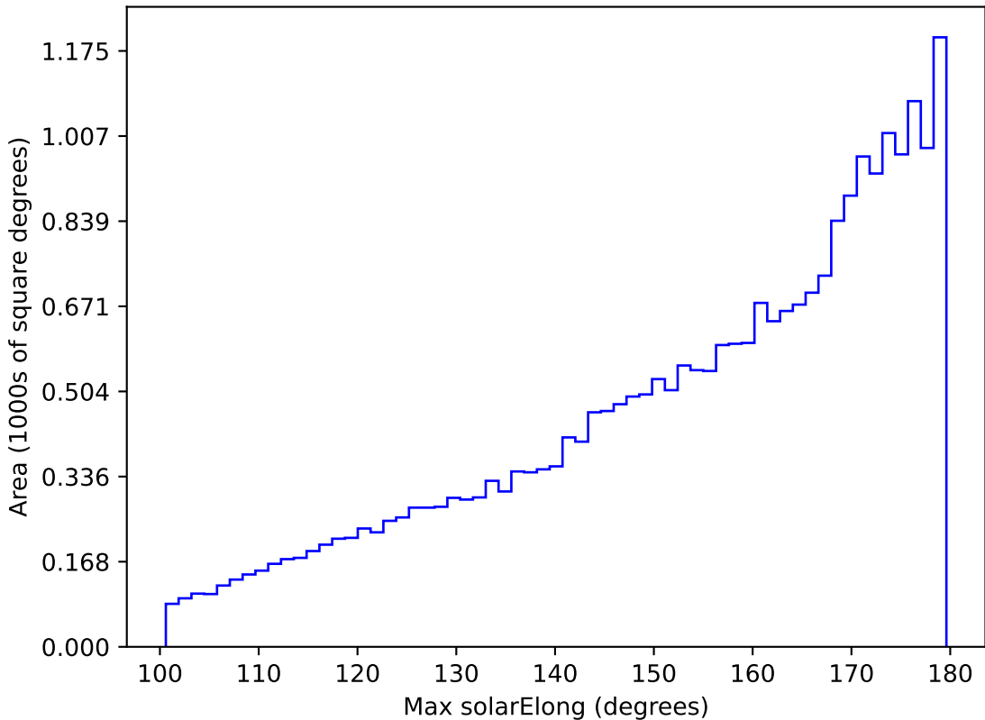
weather_cloudso20v3.4_10yrs All sky all bands: Max solarElong
