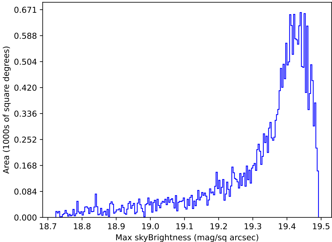
weather_cloudso20v3.4_10yrs Yr 1 z band: Max skyBrightness
