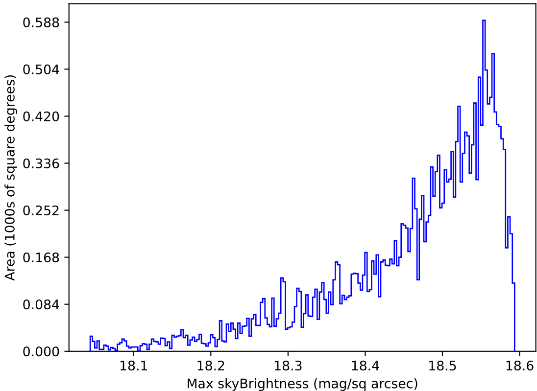
weather_cloudso20v3.4_10yrs Yr 1 y band: Max skyBrightness
