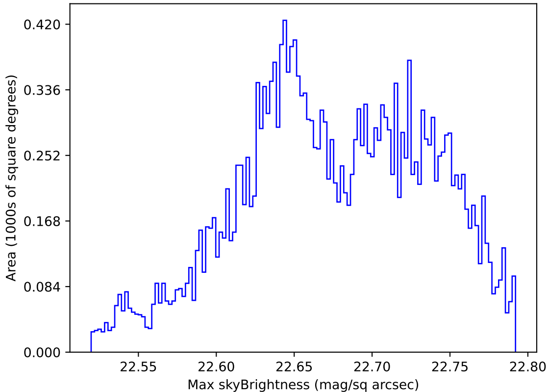
weather_cloudso20v3.4_10yrs Yr 1 u band: Max skyBrightness
