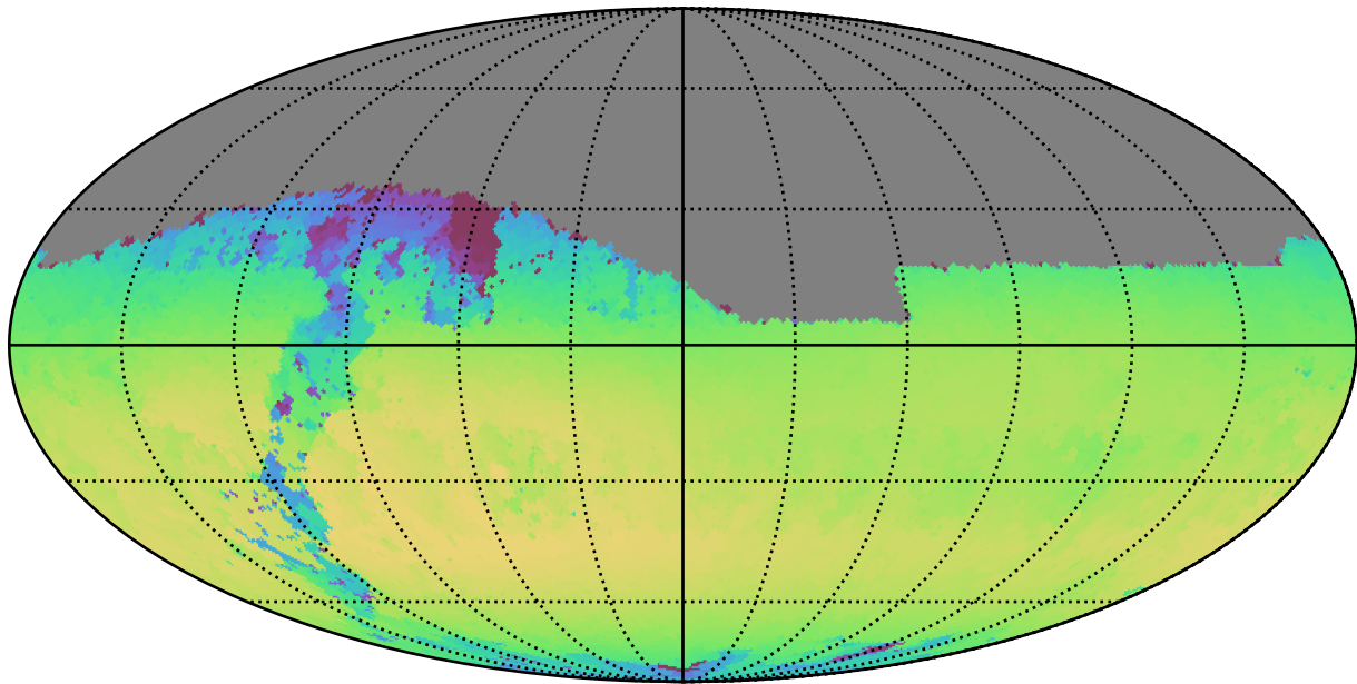
weather_cloudso20v3.4_10yrs Yr 1 i band: Max skyBrightness
