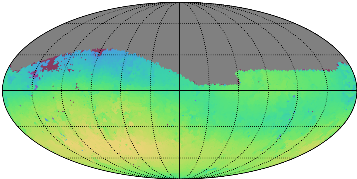
weather_cloudso20v3.4_10yrs Yr 1 g band: Max skyBrightness
