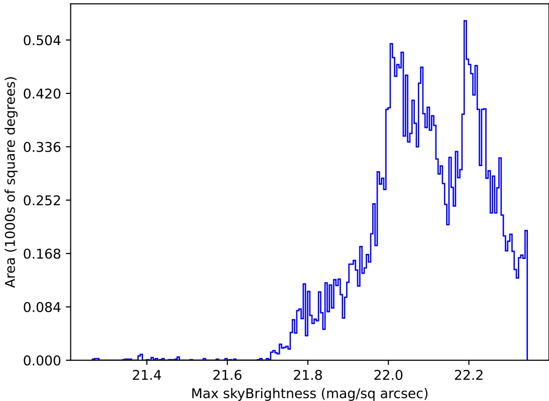
weather_cloudso20v3.4_10yrs Yr 1 g band: Max skyBrightness
