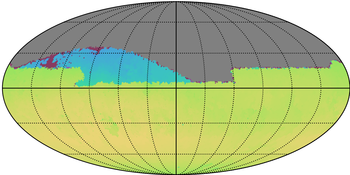
weather_cloudso20v3.4_10yrs Yr 1 all bands: Max skyBrightness
