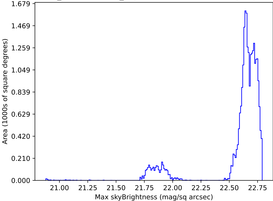
weather_cloudso20v3.4_10yrs Yr 1 all bands: Max skyBrightness
