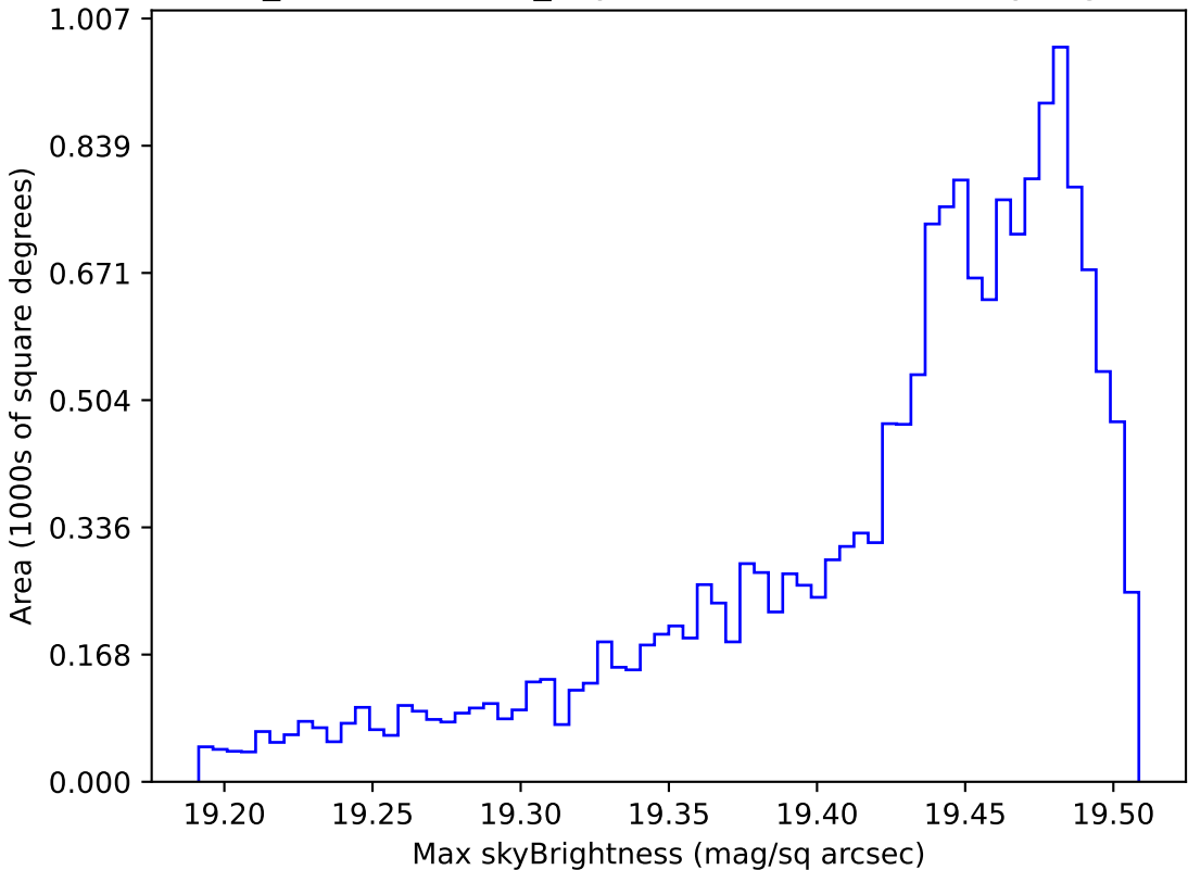
weather_cloudso20v3.4_10yrs WFD z band: Max skyBrightness
