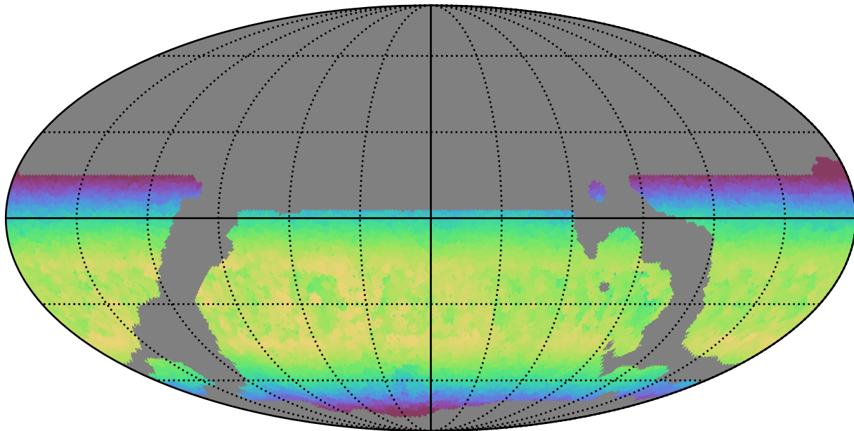
weather_cloudso20v3.4_10yrs WFD y band: Max skyBrightness
