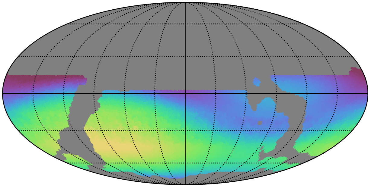
weather_cloudso20v3.4_10yrs WFD r band: Max skyBrightness
