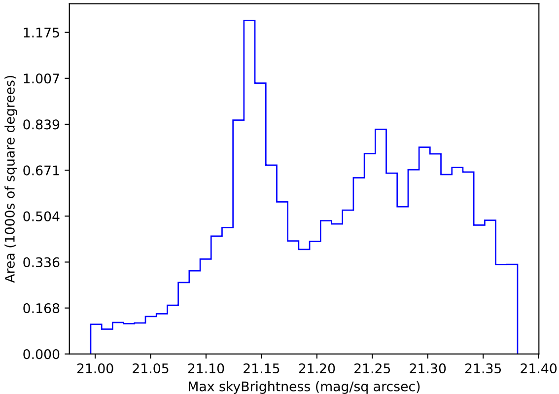
weather_cloudso20v3.4_10yrs WFD r band: Max skyBrightness
