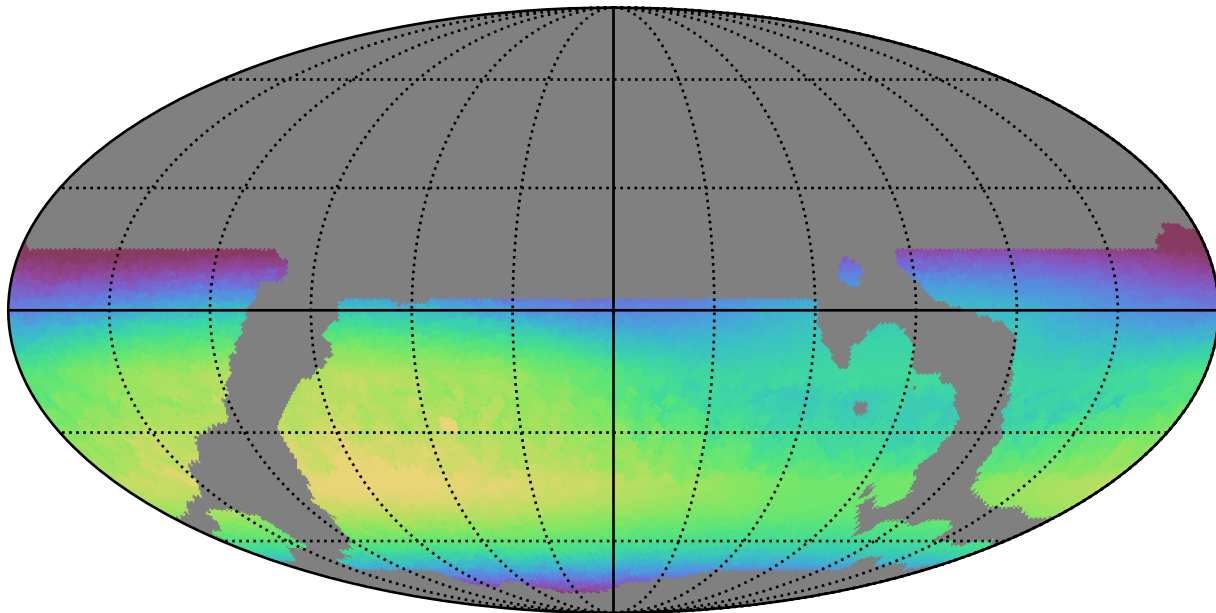
weather_cloudso20v3.4_10yrs WFD i band: Max skyBrightness
